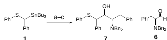
Scheme 2. a) n BuLi (1.15 equiv), cumene, –78 °C; b) ligand (1.2 equiv), –78 °C, 1 h; ( dl )- 6 or ( S )- 6 , –78 °C.
